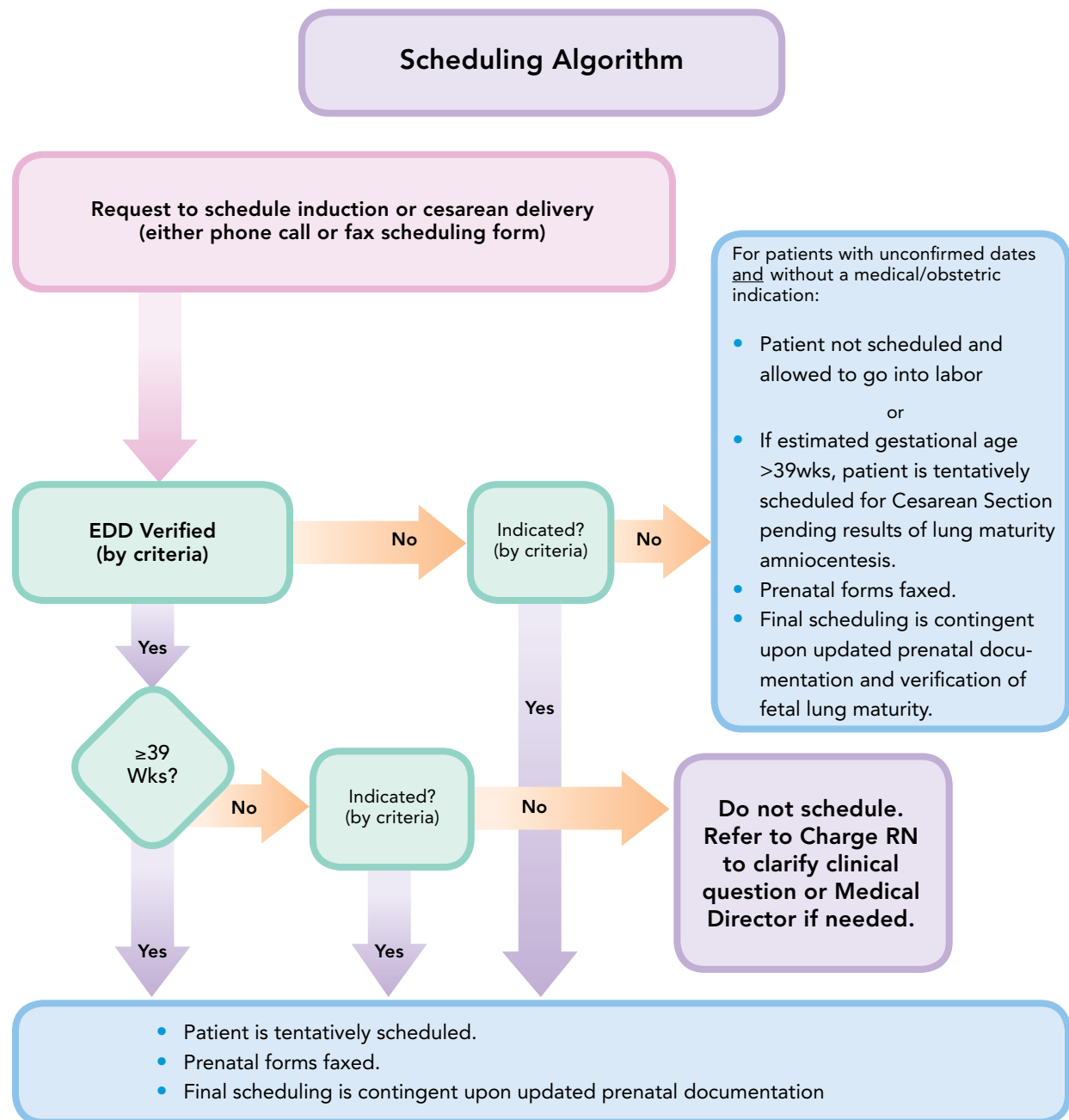
Figure 15: Scheduling Algorithm
